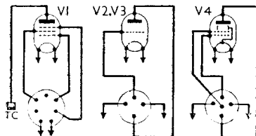
Diagrams of the four valves used.
