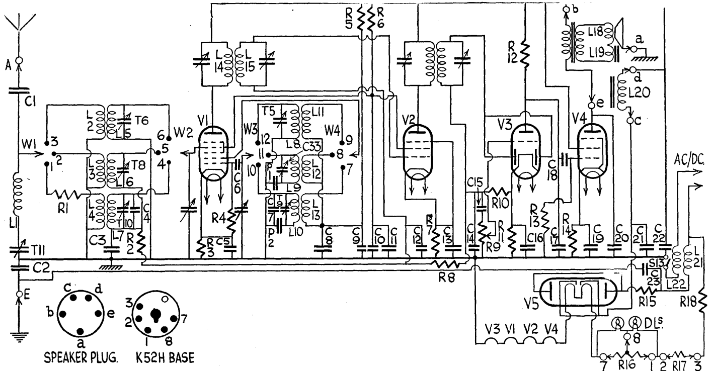
An orthodox “short” superhet circuit is found in the 600. The aerial circuit includes an I.F. trap. R16 and R17 cons is of an American K52H resistance tube.
