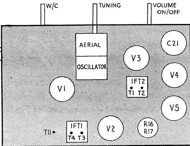
Details of the Belmont 600 chassis are given by these drawings of the top (left) and underside (right). Note the switch, coil and trimmer section on the underside.
