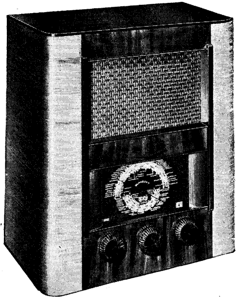
The model 267 four-band five-valve A.C. superhet made by Burndeft Ltd. of Light Gun Factory, Erith, Kent.
