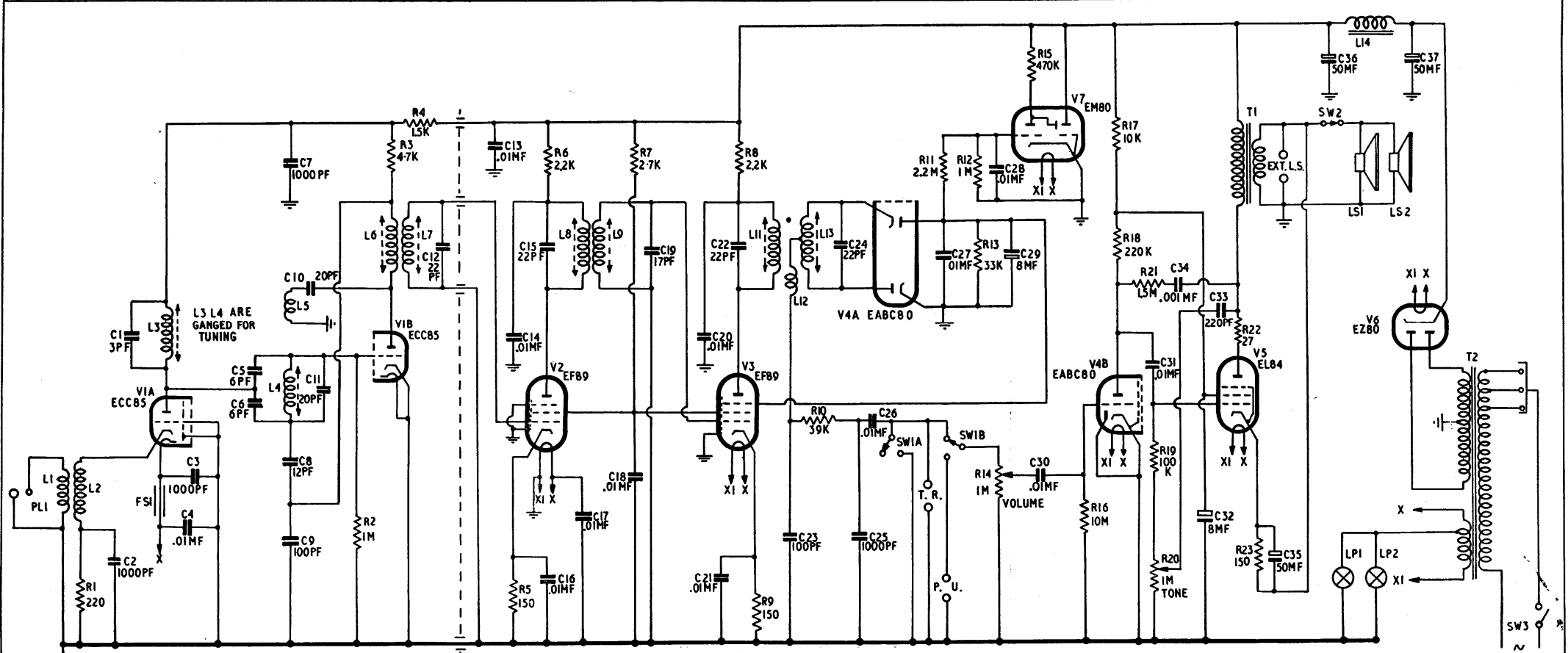
CIRCUIT DIAGRAM
