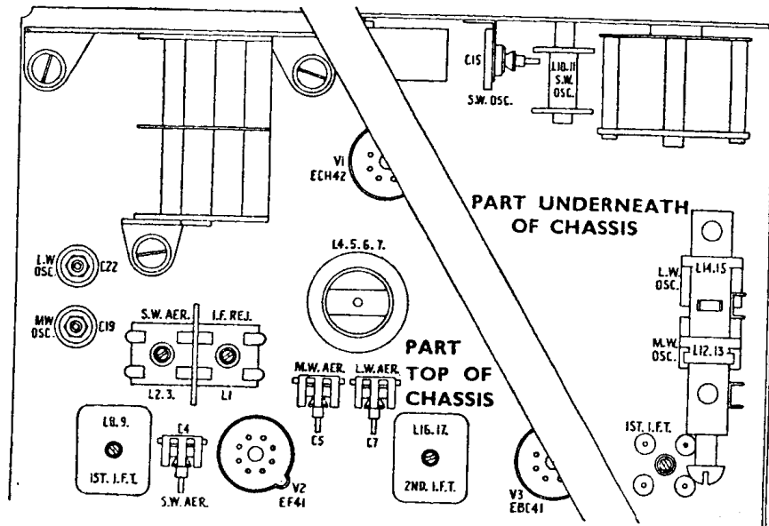
LAYOUT OF TRIMMERS
