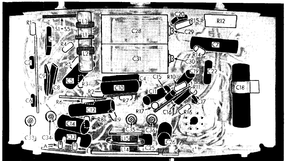
Under-chassis view. Most of the components are grouped in four assemblies.
