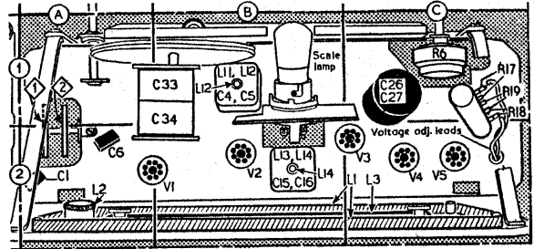
Above: Plan view of the chassis showing the voltage adjustment leads on the ballast resistor. The lower lead actually consists of a loop of wire connected as indicated under "Voltage Alignment" in "General Notes."
