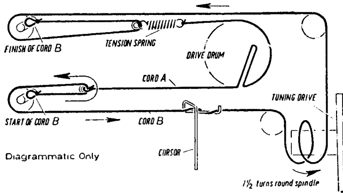
(Right) TUNING DRIVE CORD, SHOWN WITH TUNING GANG FULLY CLOSED
