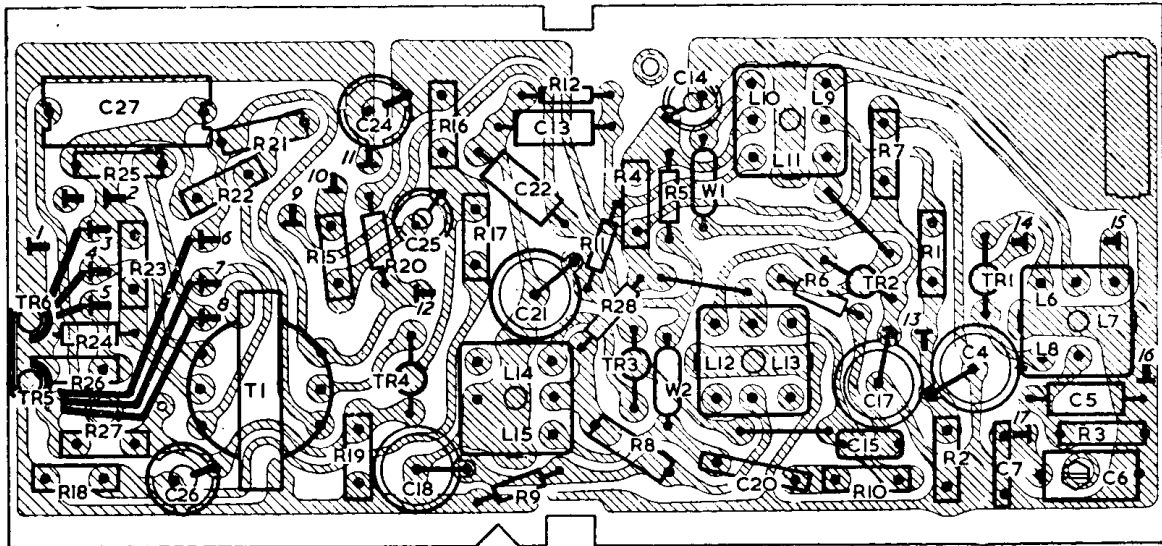
Above) PRINTED WIRING BOARD
