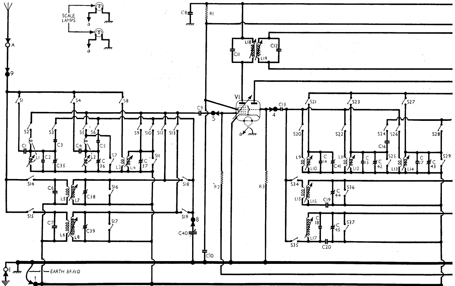
Circuit diagram of the H.M.V. 1120 5-band A.C. superhet. The S.W. bands, reading from left to right in both aerial and oscillator circuits, are S.W.3, S.W.2 and S.W.1, the lowest wavelengths being in the S.W.3 range. Electrical band-spreading is effected on S.W.3 and S.W.2 in the aerial circuit by coil tapings and series capacitors C3 and C5 ; and in the oscillator circuit by C22 (S.W.3) and C16 (S.W.2). The numbers 1 to 9 around the aerial and oscillator circuits indicate the points of inter-connection between the tuning assembly and the rest of the chassis.
