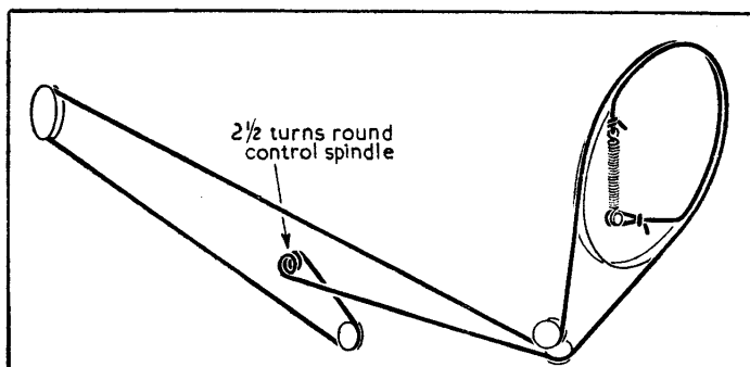
Sketch showing the tuning drive cord system, drawn as seen from the front right-hand corner of the chassis when the gang is at minimum capacitance.
