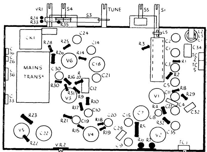
These diagrams show (left) how the components are arranged on the top of the 219 chassis, and (right) the "below deck" arrangement. Reference is made to the mechanical silencing switch under "Special Notes" on the previous page.
