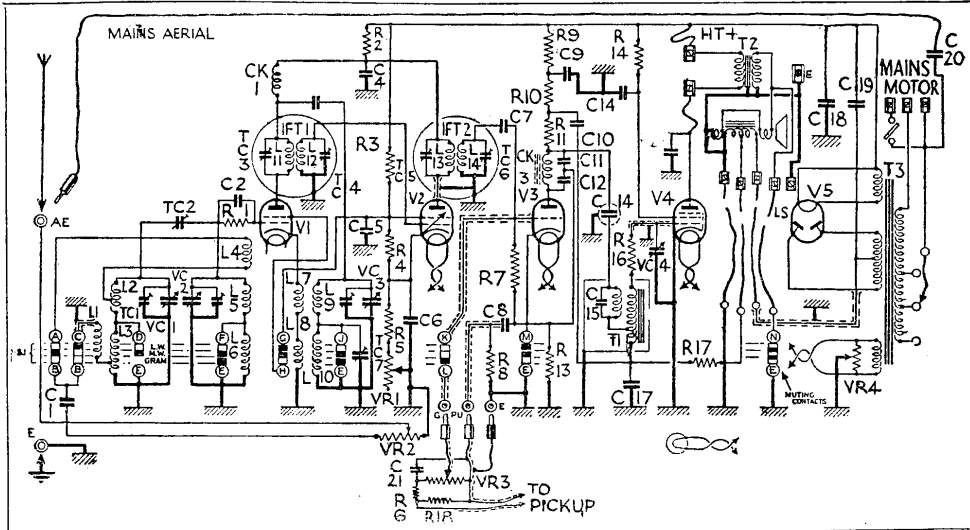
In some models the detector anode circuit choke CK3 is replaced by a 10,000 ohm resistance. If the motor terminals are lettered A.B.C. the right-hand one goes to the 231-250 volt mains transformer tapping.
