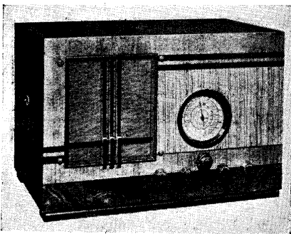
The model 345 receiver by Marconiphone is a 6-valve A.C. mains superhet with provision for four wavebands.
