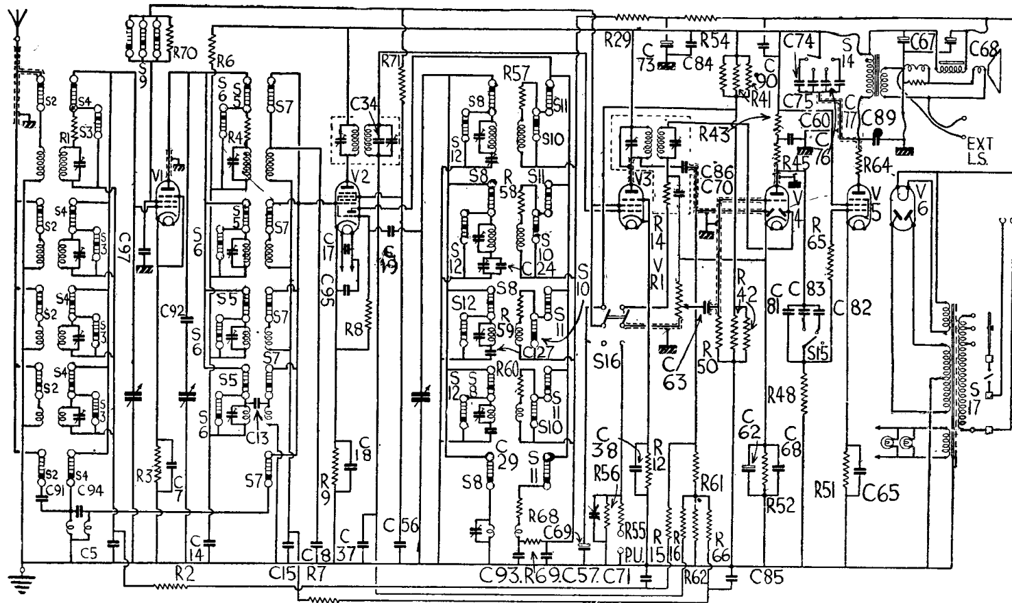
A complete guide to the circuit of the Marconiphone 346 all-wave superhet A.C. five is given in the circuit diagram below and the tables of component values above.
