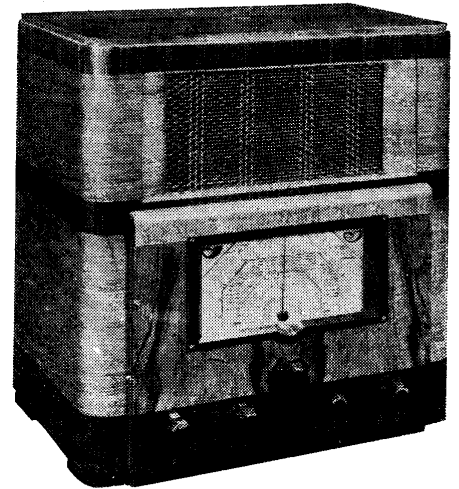
The 538 is a seven-valve, plus rectifier, four-band superhet.
