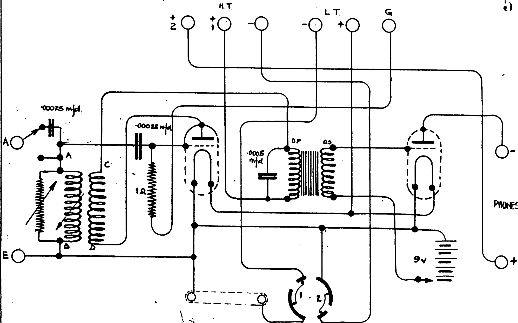
Schematic Diagram of Receivers Type 21.
