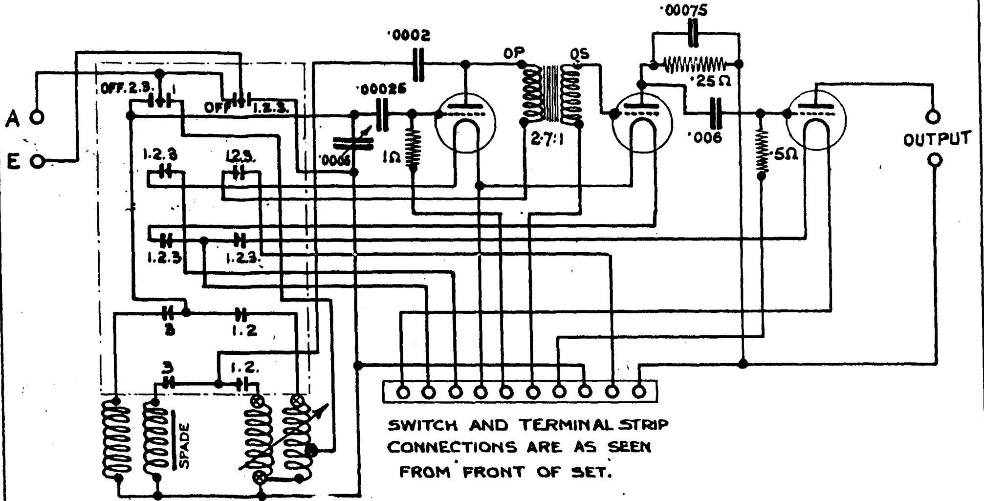
DIAGRAM OF CONNECTIONS RECEIVER. TYPE 32.
