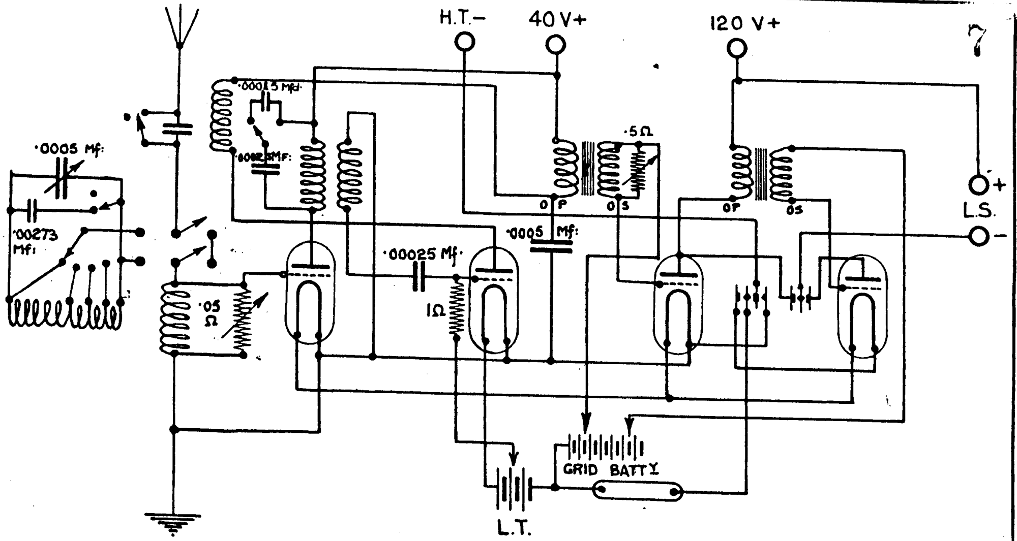
DIAGRAM OF CONNECTIONS RECEIVER TYPE 41
