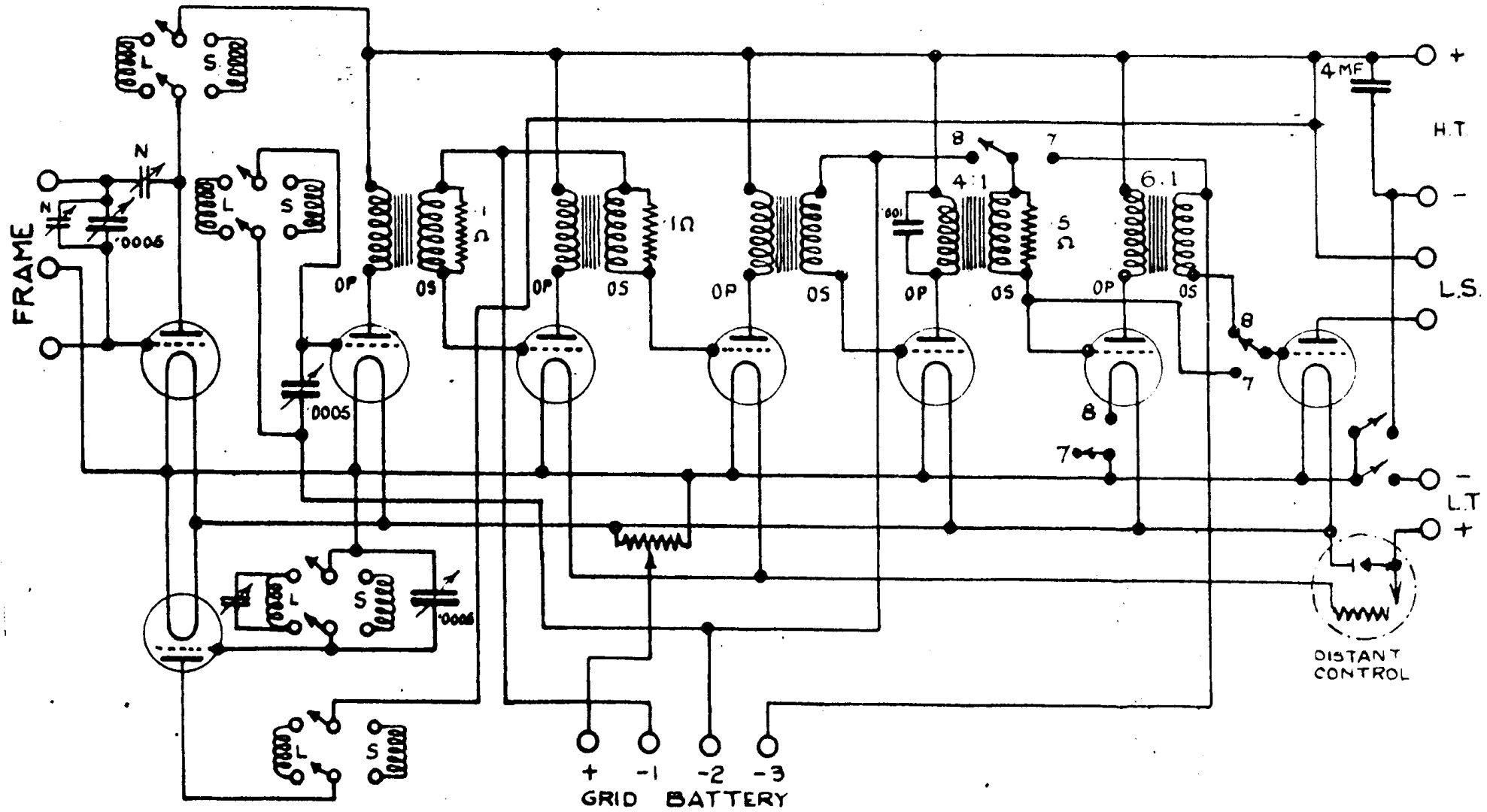
DIAGRAM OF CONNECTIONS RECEIVER TYPE 82
