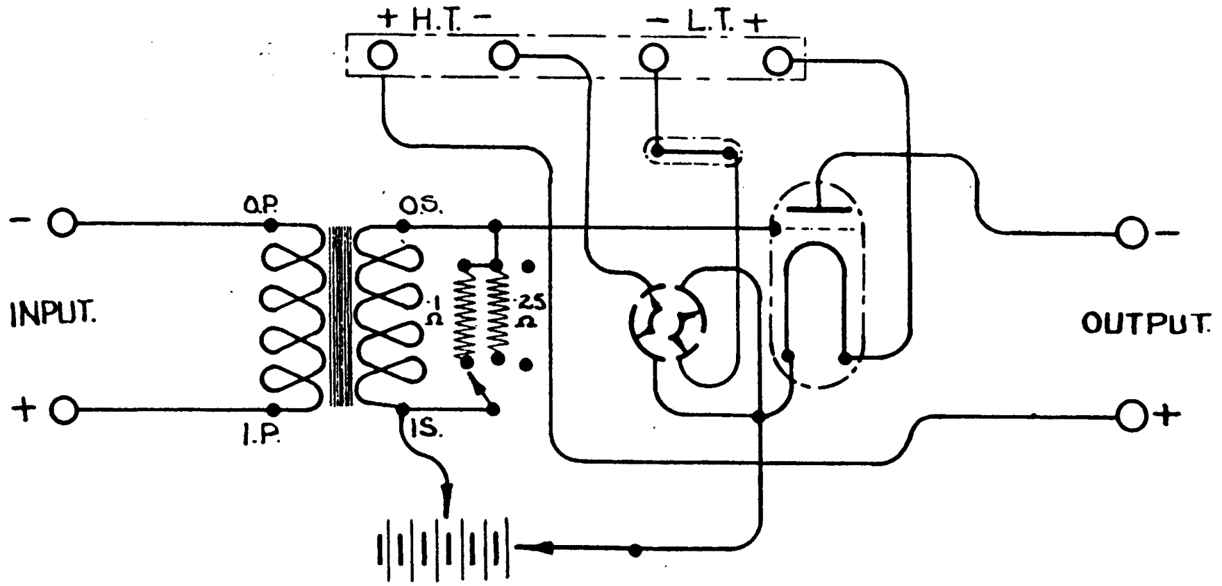
SCHEMATIC DIAGRAM OF L.F. AMPLIFIER TYPE N° A4.
