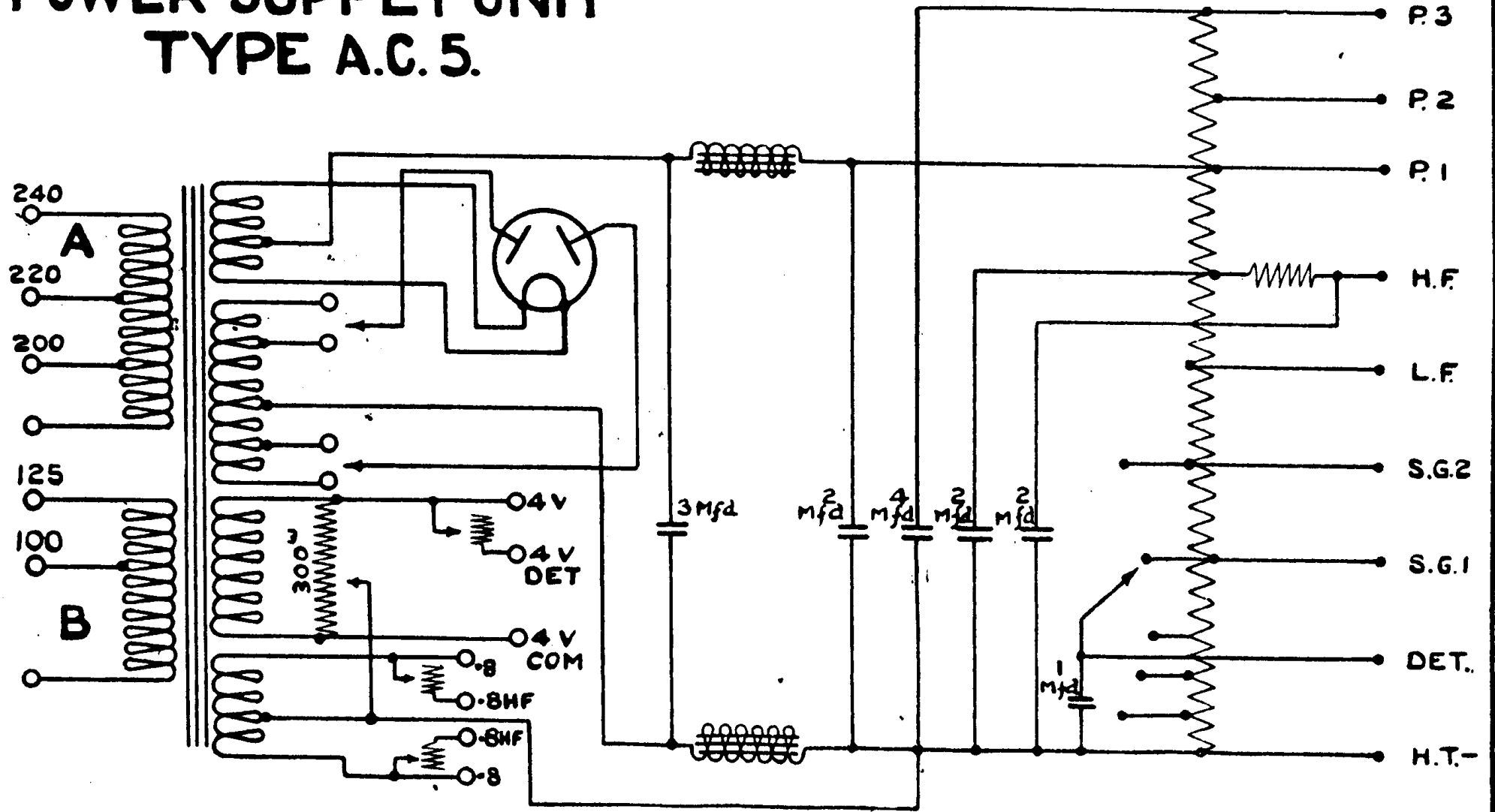
A & B ALTERNATIVE WINDINGS
