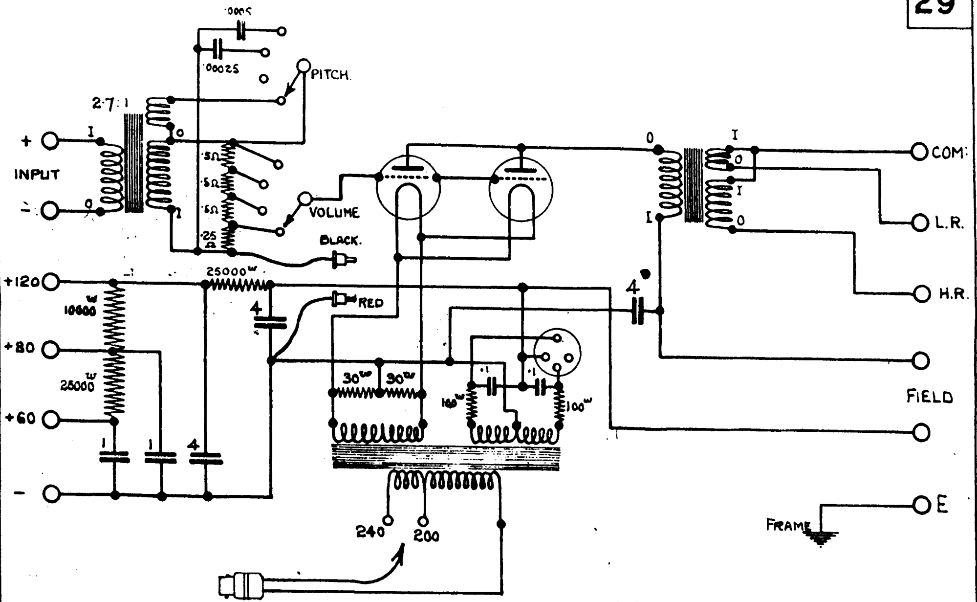
DIAGRAM OF CONNECTIONS AMPLIFIER TYPE A.C.A.
