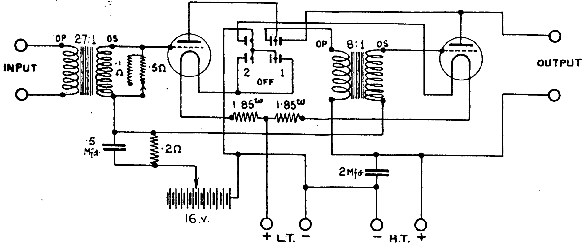
DIAGRAM OF CONNECTIONS.
