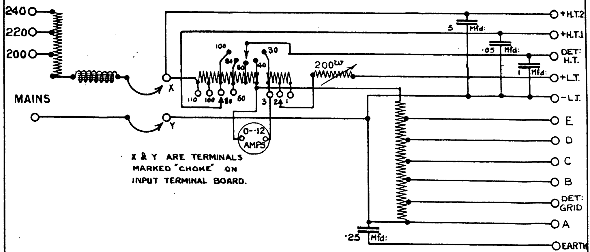
DIAGRAM OF CONNECTIONS ALL POWER SUPPLY UNIT. TYPE D.C.1. (EDN: A)
