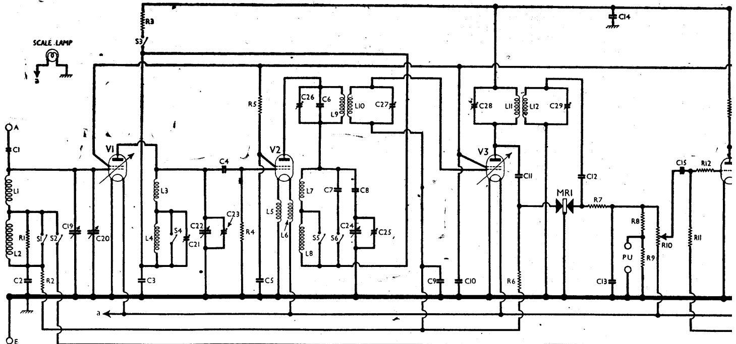
Circuit diagram of the Marconiphone 269 portable battery superhet. The HMV 462 employs an identical chassis. MR1 is the metal rectifier for V1 and V2, while S2 closes to bias up V1 and reduce screen current. L5, L6 are the oscillator reaction coils, in the filament circuit of V2. T
