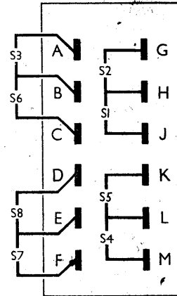
Diagram showing the connections to the switch unit, drawn as seen in the position indicated in our under-chassis view.
