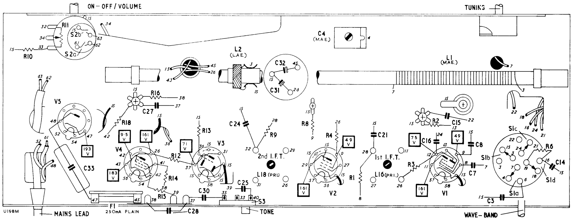
Fig.3. Chassis underside of later U198M receivers. The chassis top is as shown in the U198H Manual.
