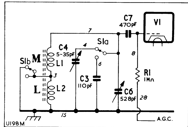
Fig.2. U198M modified aerial circuit.
