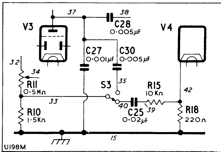
Fig.1. U198M modified tone control circuit.
