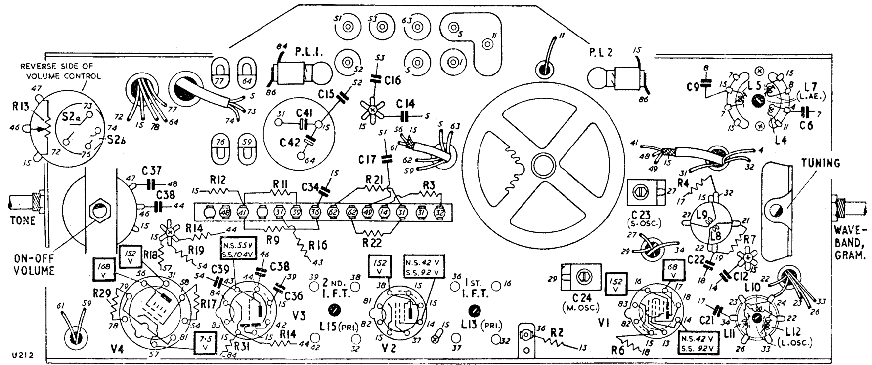
The layout of the front and rear of the chassis
