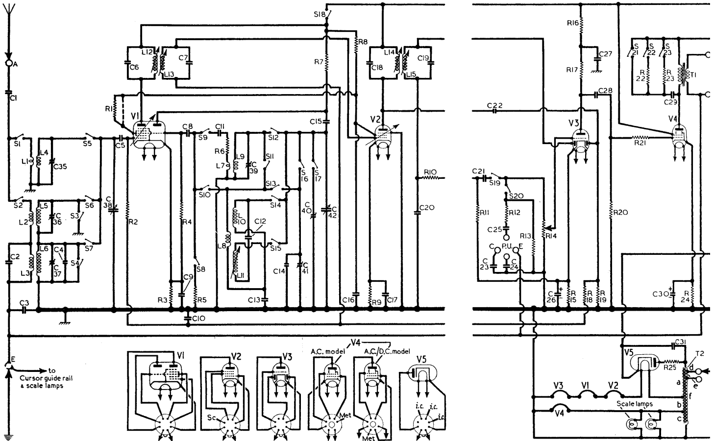
R.F., oscillator and I.F. circuits of the 130 series, which is common to both A.C. and A.C./D.C. versions. The dotted line to V1 screen indicates that R1 is omitted in the U130.
