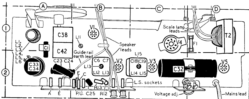
Plan view of the A.C. chassis. Attention is drawn to the special earthing facility for the cursor guide rail and scale lamp housings on the split E socket.
