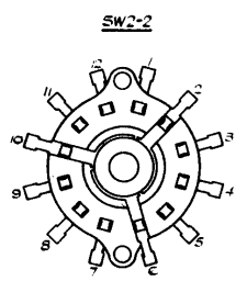
VIEWS OF SWITCHES FROM FRONT CHASSIS BEING UPSIDE DOWN
