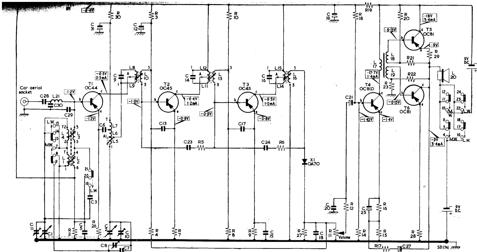
CIRCUIT DIAGRAM—PHILIPS MODEL L3Go3T
