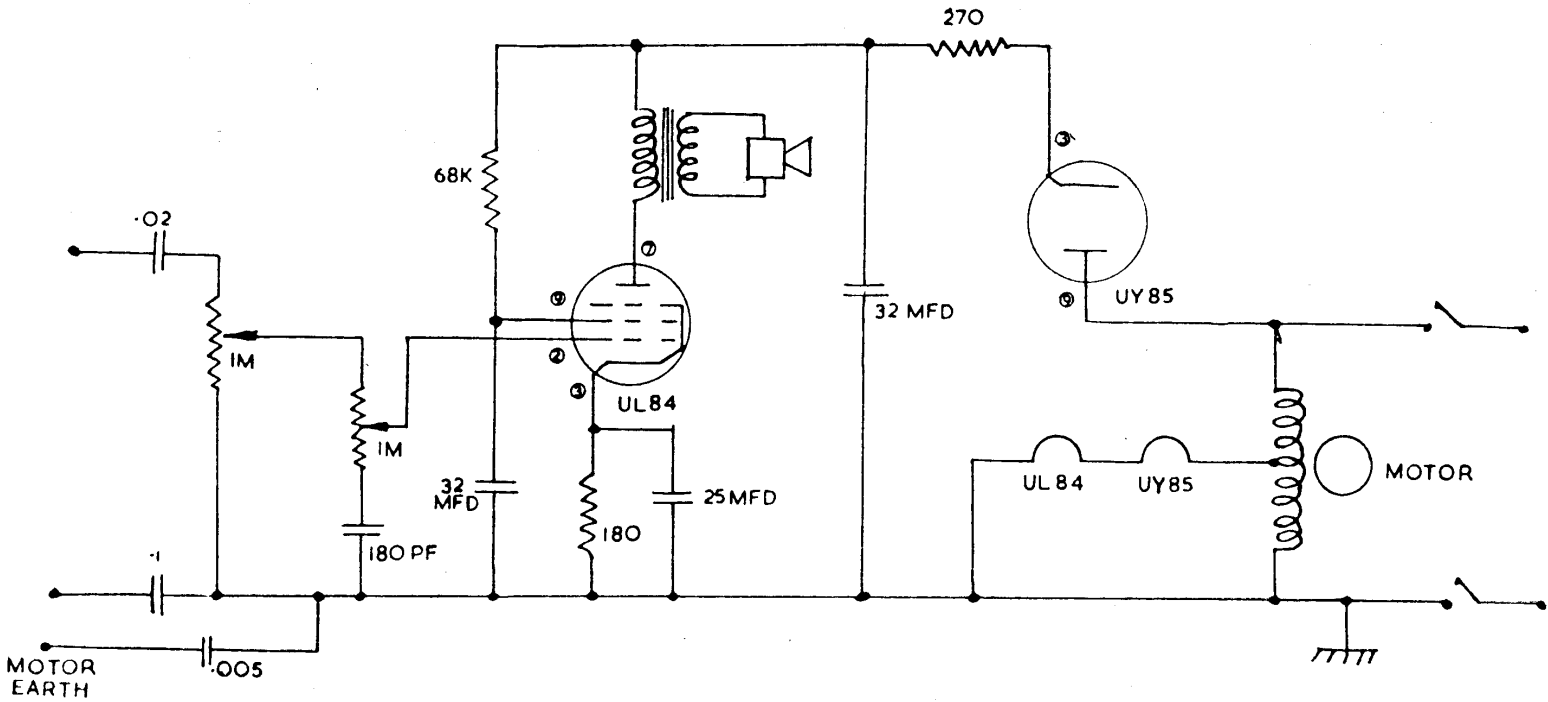
CIRCUIT DIAGRAM—PORTADYNE RECORD PLAYERS MODELS RP10, RP11, RP12, RP15
