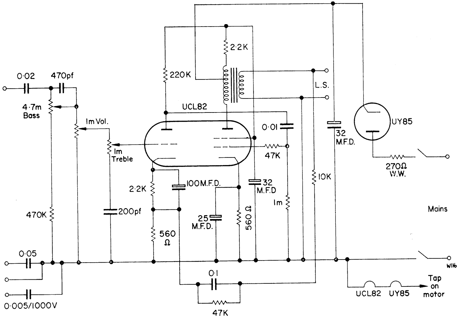
(W116) CIRCUIT DIAGRAM—MODELS RP17 AND RP20
