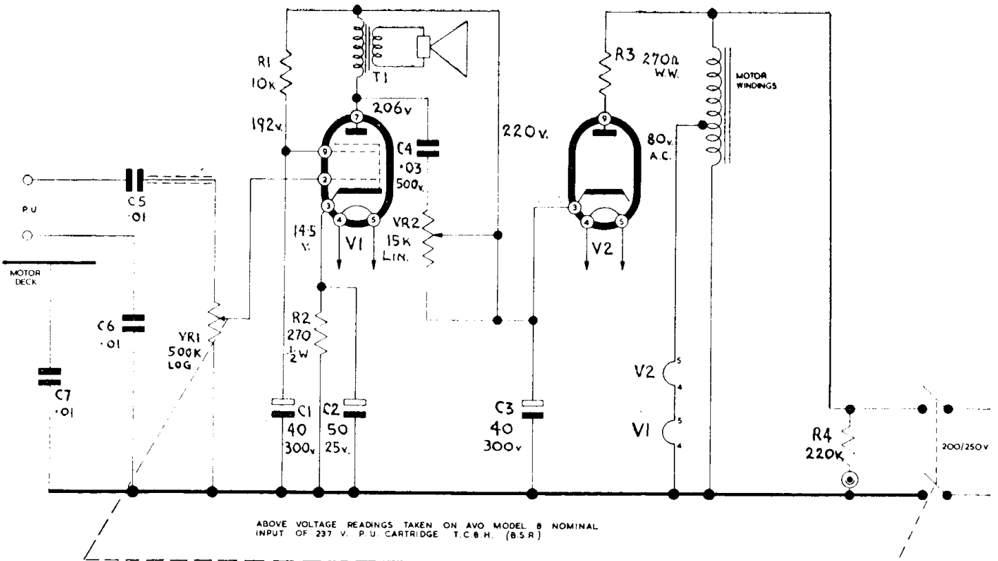
CIRCUIT DIAGRAM—REGENTONE MODEL AHG II
