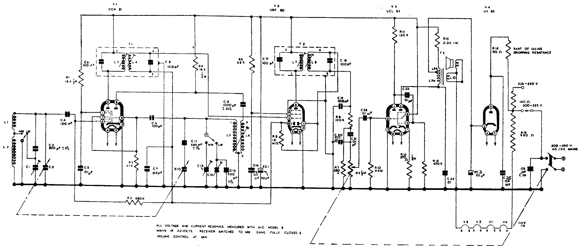
CIRCUIT DIAGRAM—REGENTONE MODEL D15
