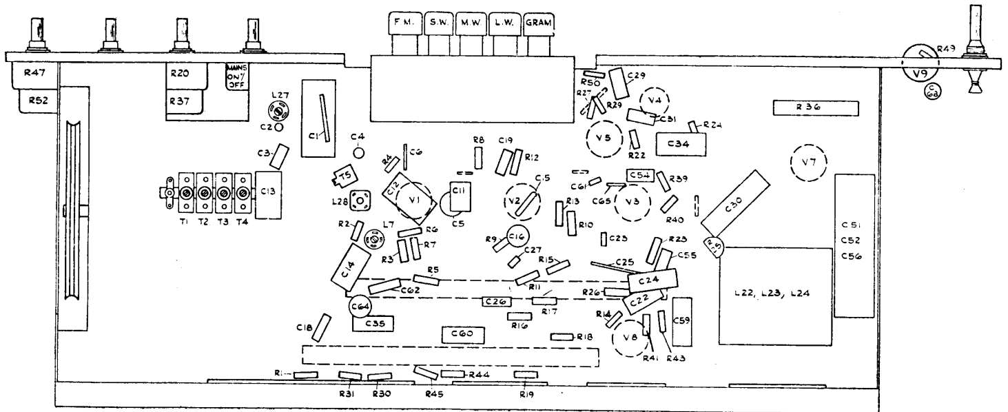
COMPONENT LAY-OUT DIAGRAM—REGENTONE MODEL SRG25
