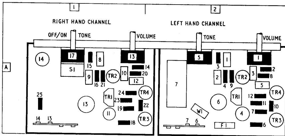
Component locations viewed from component side of circuit panels
