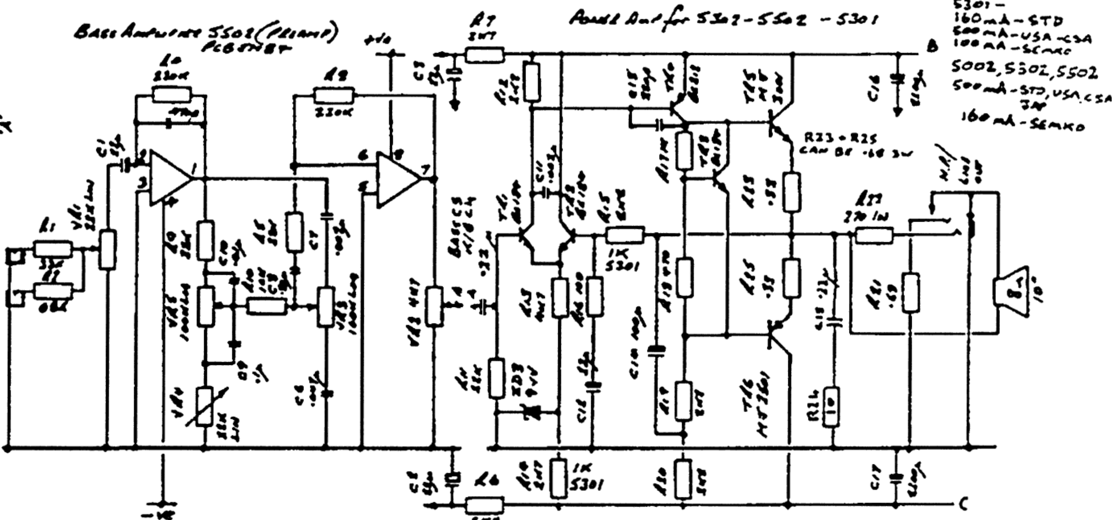
MARSHALL 20Watt Combo Series 5002, 5302, 5502. Circuit Diagram. 30-3-84 12 Watt Keyboard Combo 5301 1552 6-6-86 R.S.
