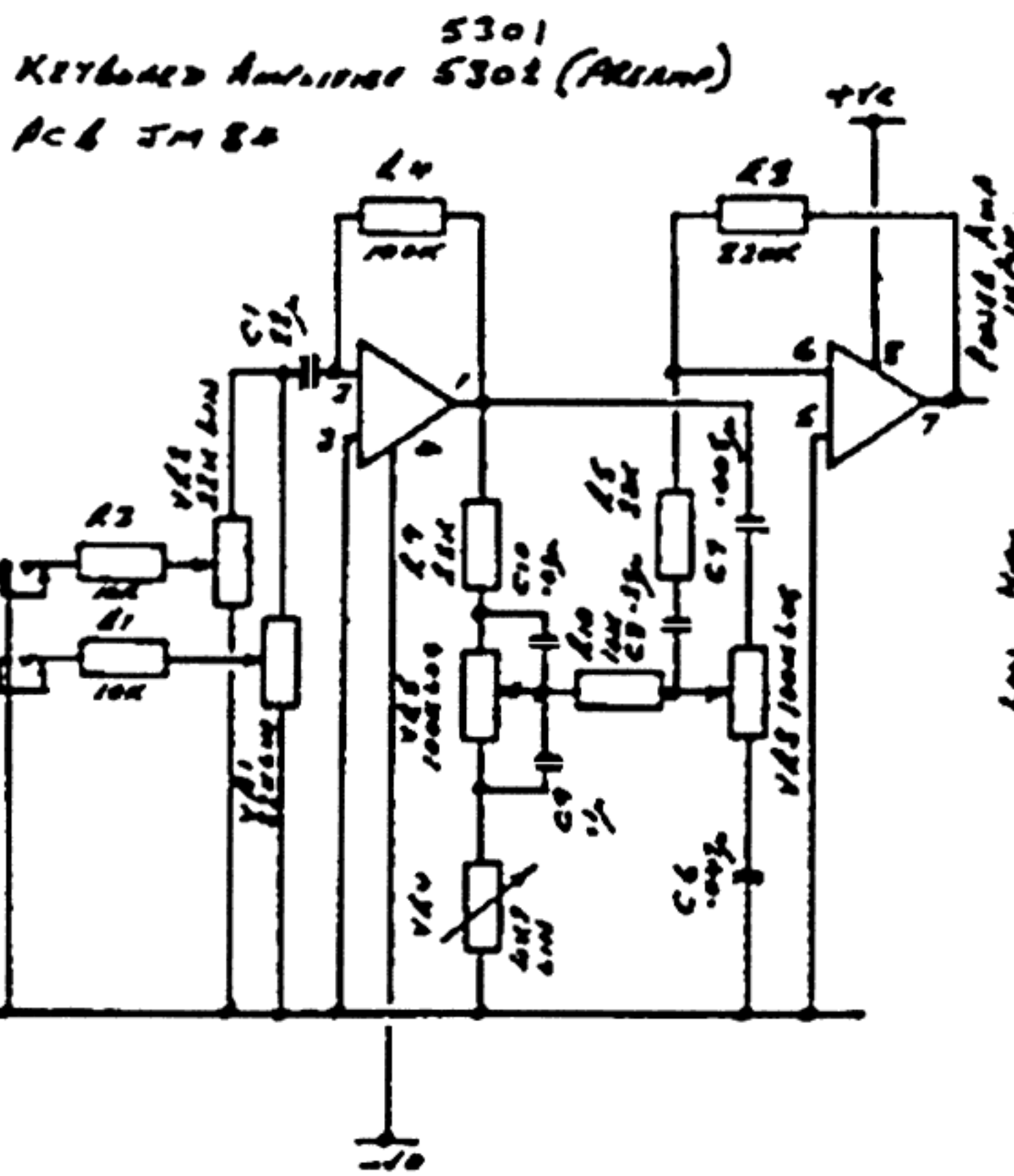
MARSHALL 20Watt Combo Series 5002, 5302, 5502. Circuit Diagram. 30-3-84 12 Watt Keyboard Combo 5301 1552 6-6-86 R.S.
