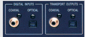
Digital input connectors
