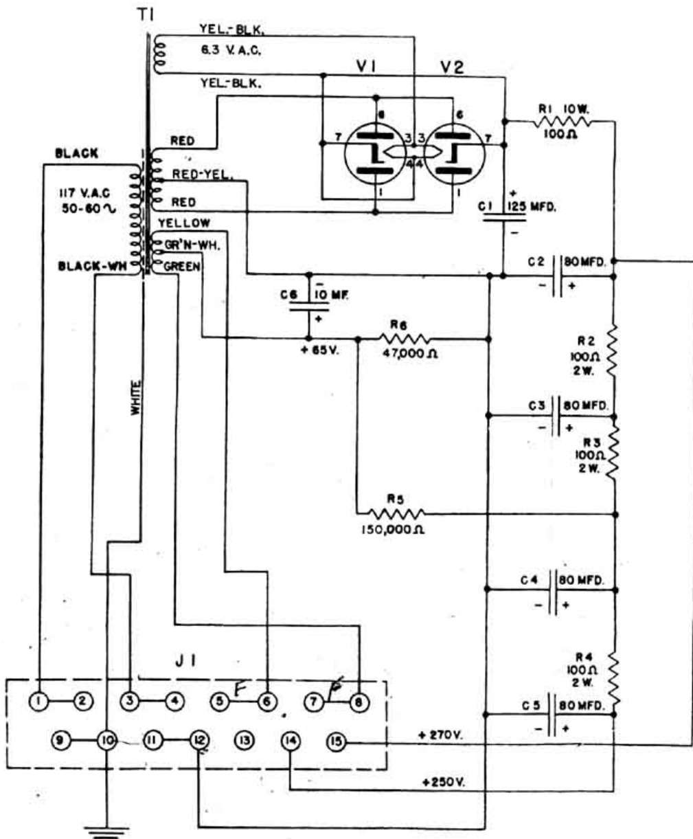
ALTEC LANSING P522B POWER SUPPLY
