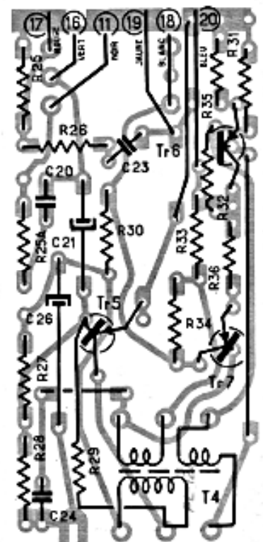
Platine BF
