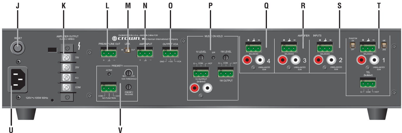
Figure 1.2 Back Panel Controls, Connectors and Indicators
