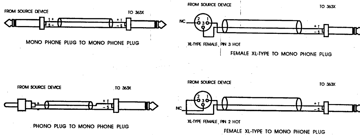
Figure 16: Input Connections
