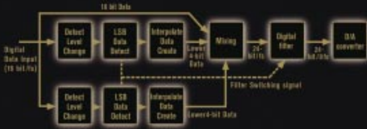
Fig.1: AL24 Processor Block Diagram
