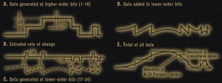
Fig.2: How AL24 Processing Works on Audio Signals
