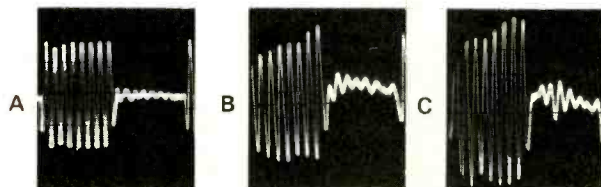
Fig. 5 —Tone burst response at A , 500 Hz; B , 8000 Hz, and C , 10,000 Hz.
