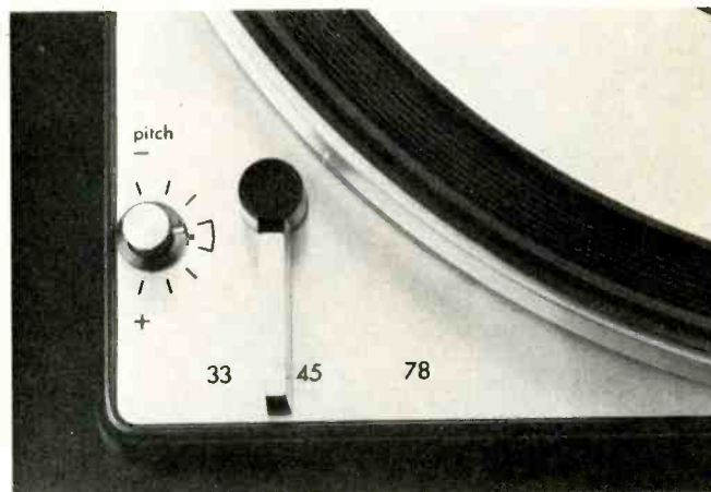
Fig. 4 —The left-front corner accommodates the speed controls—the lever for the three nominal speeds, and the knob for vernier adjustment of turntable speed over a range of \pm 3\% .
