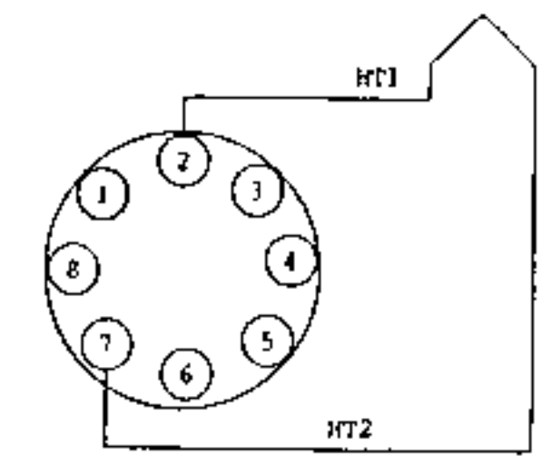
BOTTOM VIEW OF 6N3CE
