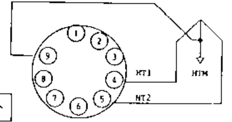
BOTTOM VIEW OF 6N2P
