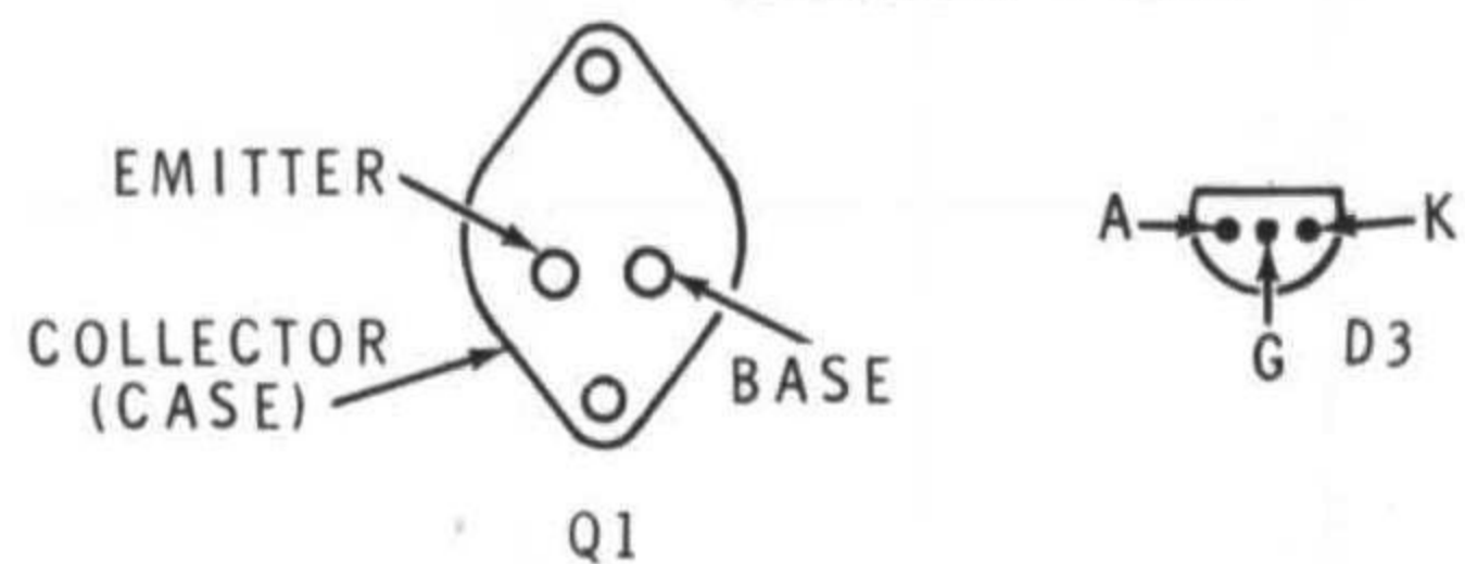
BASING DIAGRAM (BOTTOM VIEW)
