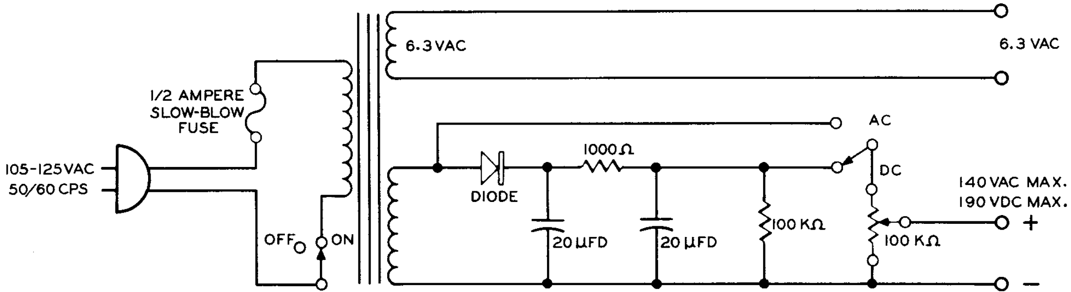
SCHEMATIC OF THE HEATHKIT® POWER SUPPLY MODEL EF-1
