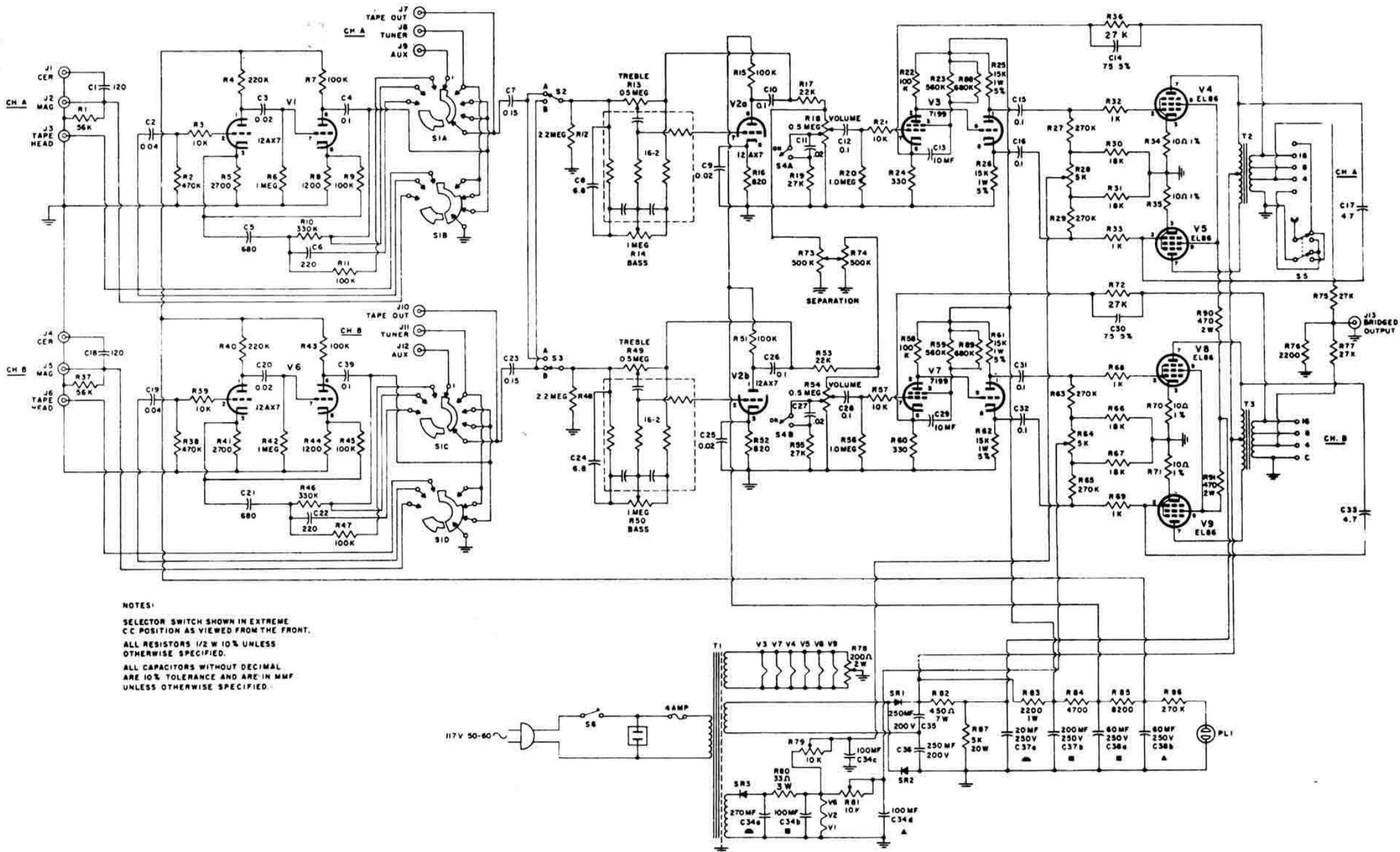
Complete schematic of the KT-250-A kit amplifier.
