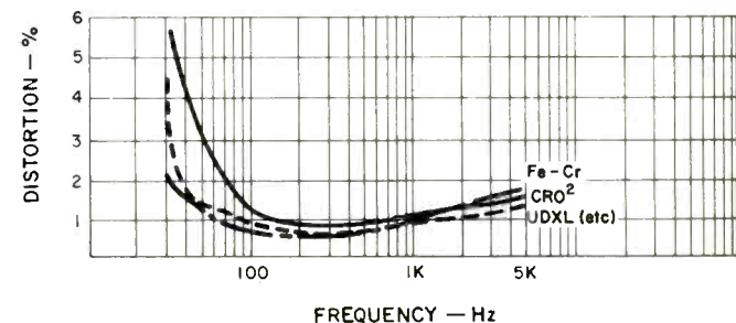
Fig. 6—Distortion vs. frequency.
