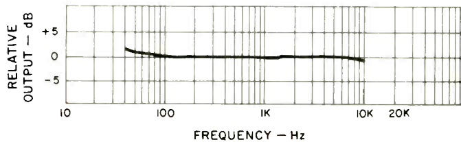
Fig. 1—Frequency response with the 40 Hz to 10 kHz test tape.
