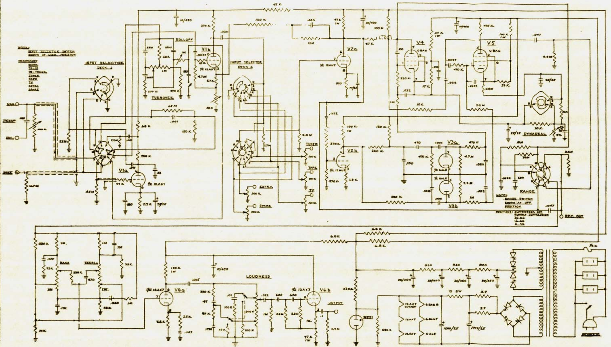
121 DYNAAURAL EQUALIZER PREAMPLIFIER CIRCUIT DIAGRAM
